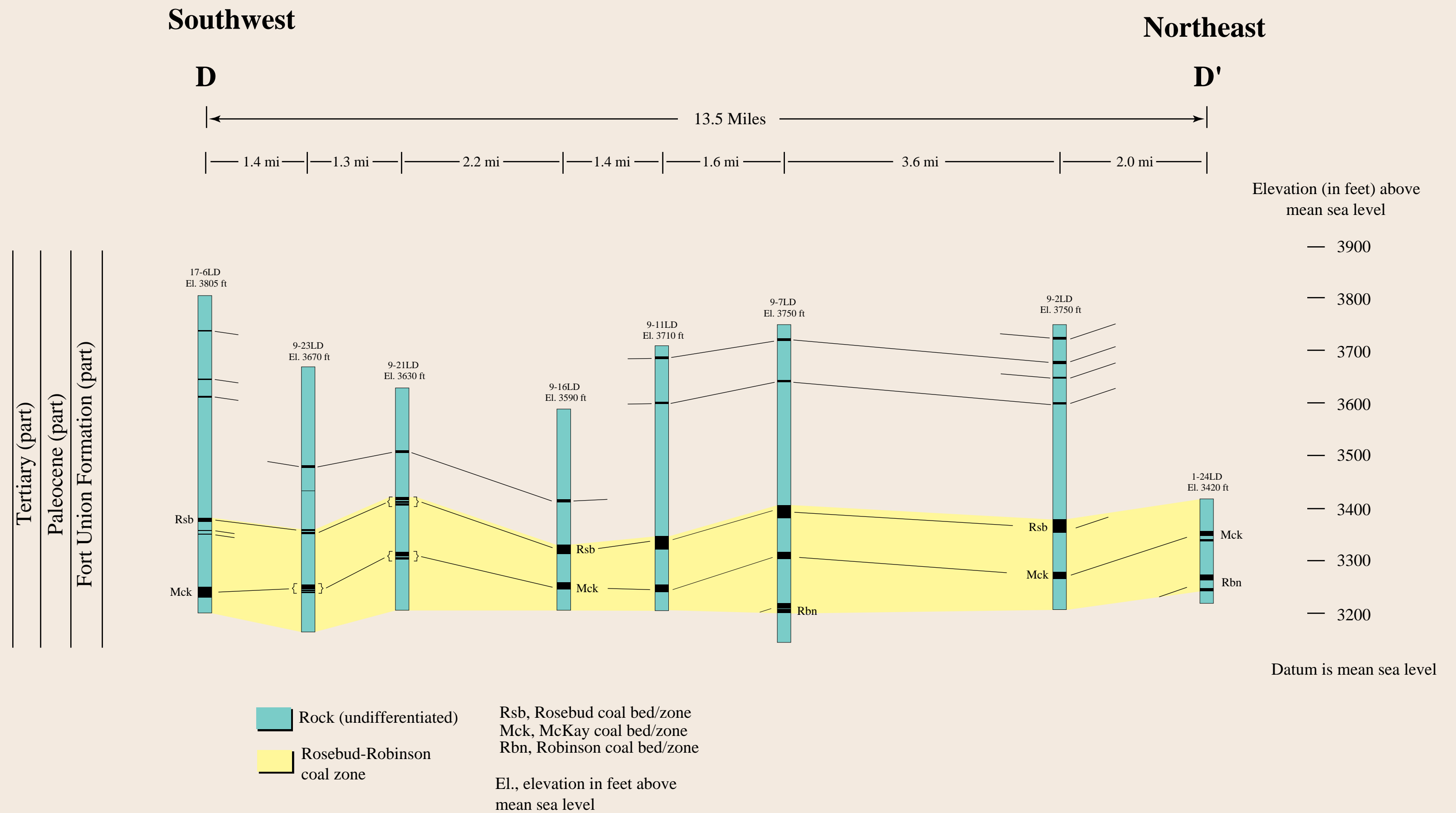
Figure PC-10. Southwest-Northeast cross section D-D', Colstrip coalfield, south-central Montana.
